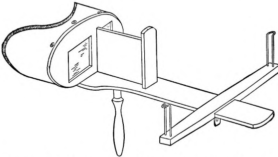
FIG. 24. — Hand stereoscope (Petzold, Mk. 8.50; Chicago Lab. Supply Co., $1.50).
