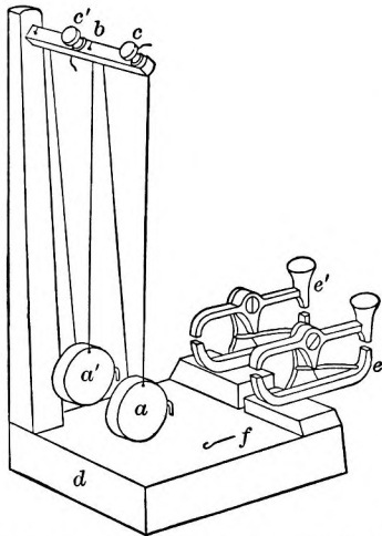
FIG. 21.—Vernier chronoscope (Clark University Lab., $5.00).
