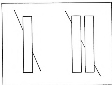
FIG. 46. — Poggendorff's illusion.
