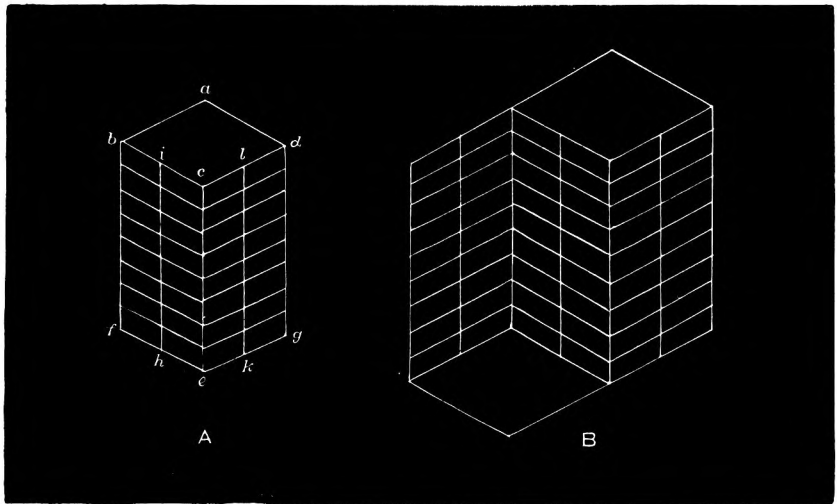
FIG. 33.—Thiéry's Prisms.
