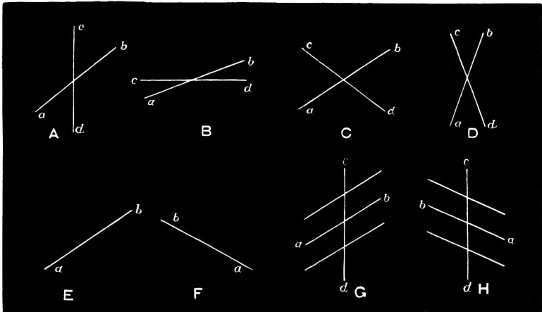
FIG. 29.—Hering's Crosses.
