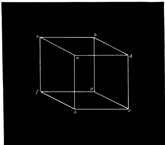
FIG. 32. — Necker's Cube.
