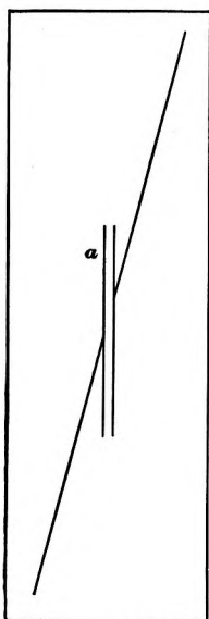
FIG. 41.—Poggen-dorff's illusion.
