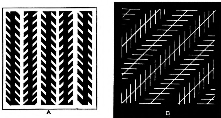
FIG. 40.—Zöllner's Figure.
