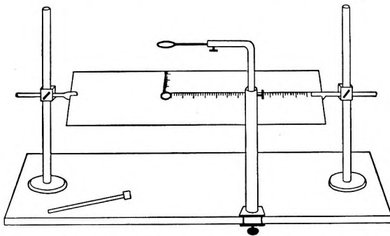
FIG. 4. — Campimeter, made by Chicago Lab. Supply Co., $4.00.
